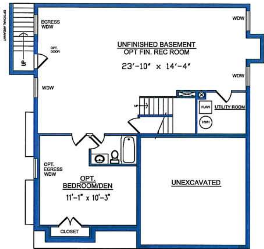
BASEMENT PLAN
