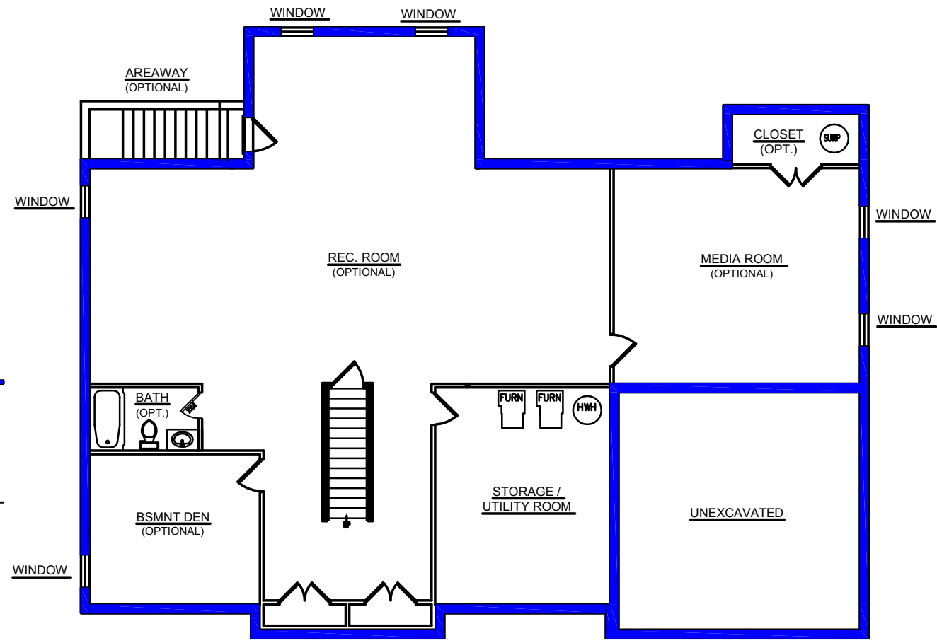
BASEMENT PLAN
