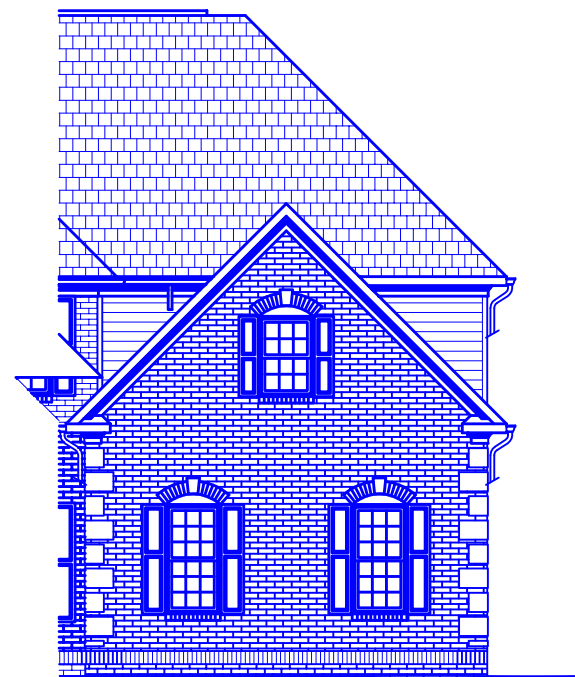
PARTIAL FRONT ELEVATION "C"
