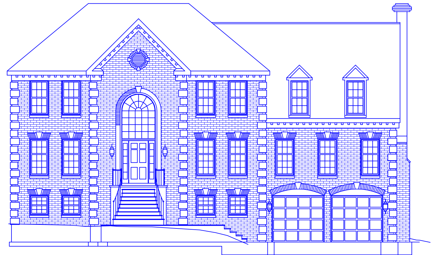
ELEV. "C" w/ optional masonry fireplace
