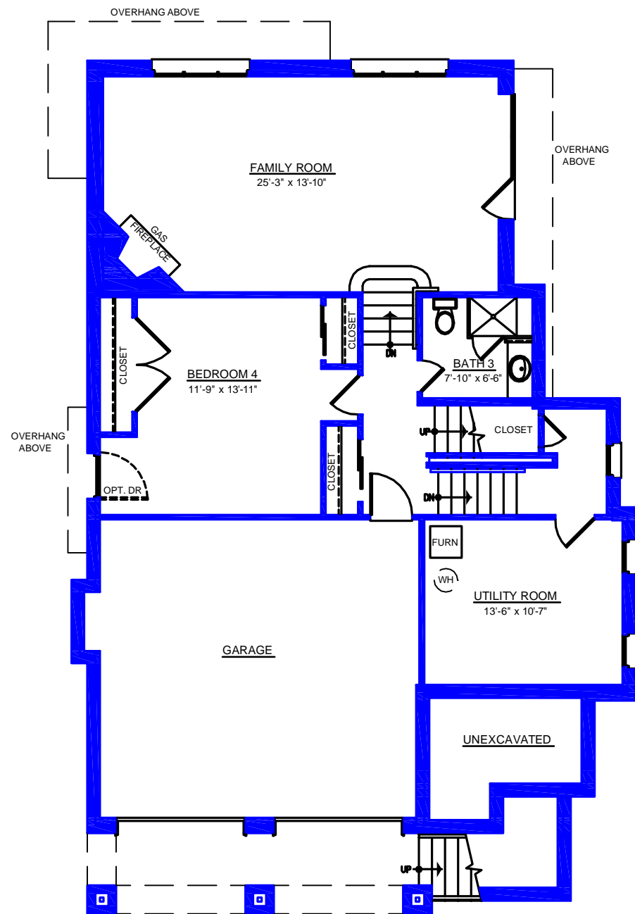
BASEMENT PLAN
