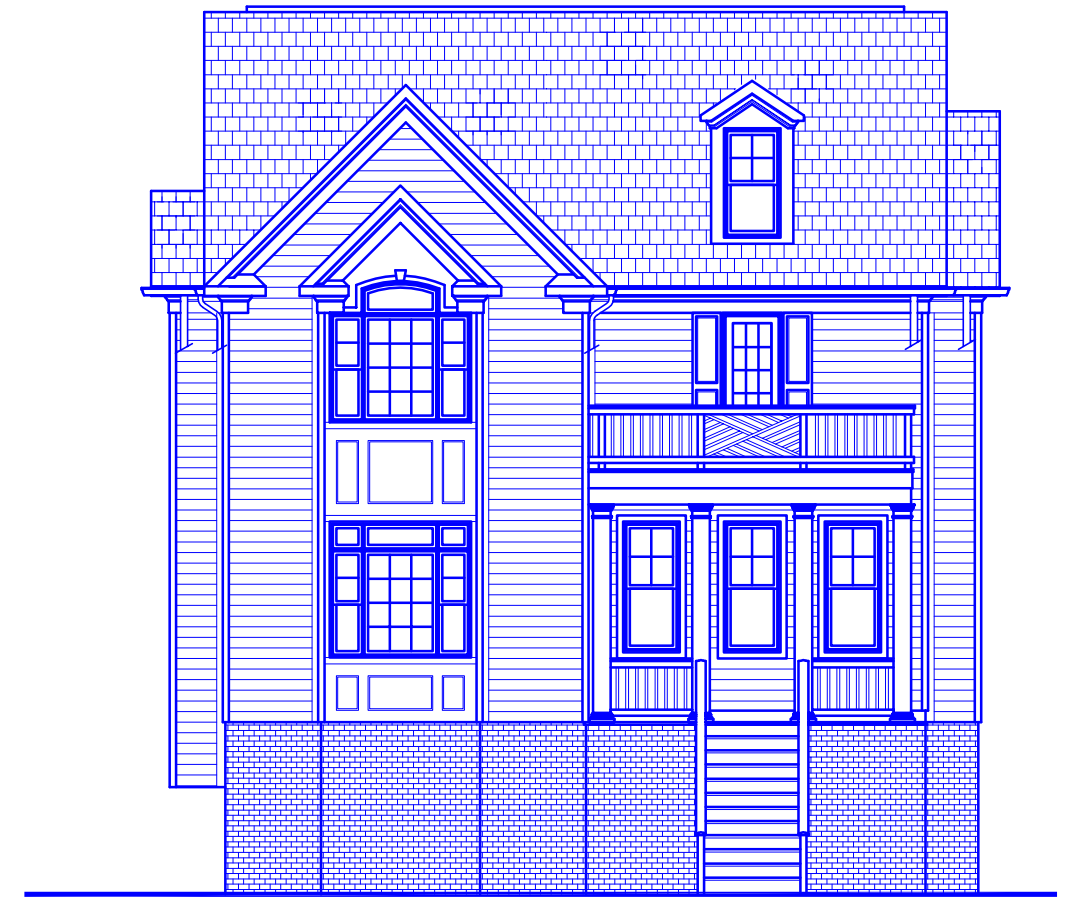
FRONT ELEVATION
